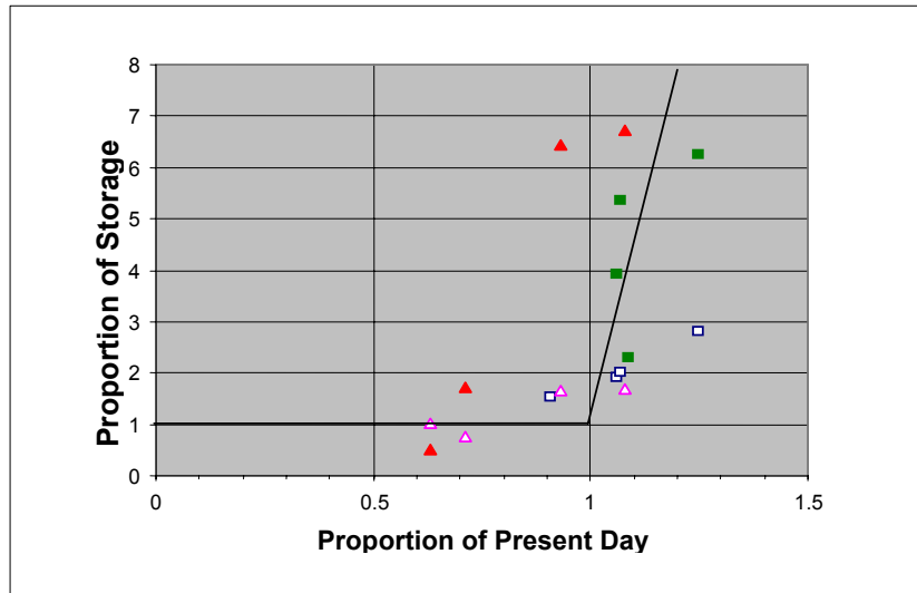
Figure 5. Correlation between Storage Volume Requirements and Rainfall for meeting Coastal CSO Discharge Standards
