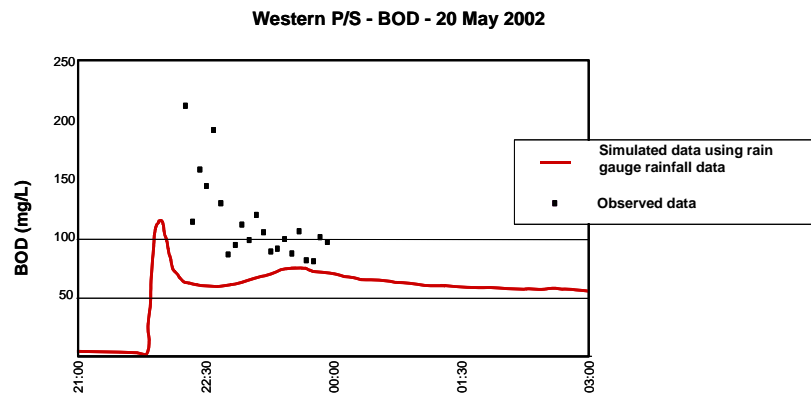
Comparison of Measured and simulated concentrations at CSO
