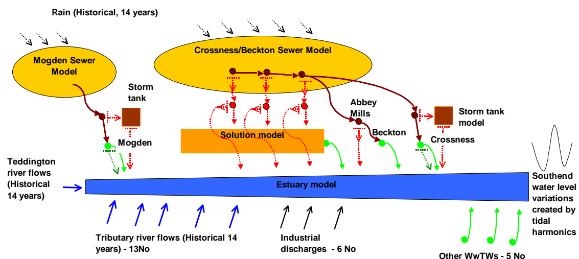
Overall Modelling framework
